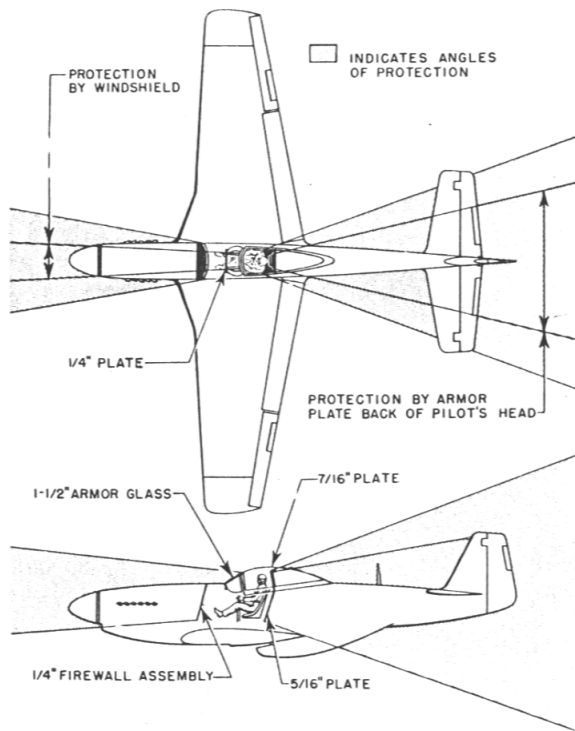
Figure 8—Armor Protection
