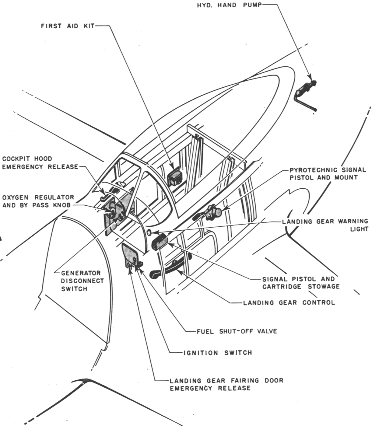
Figure 30—Emergency Equipment
