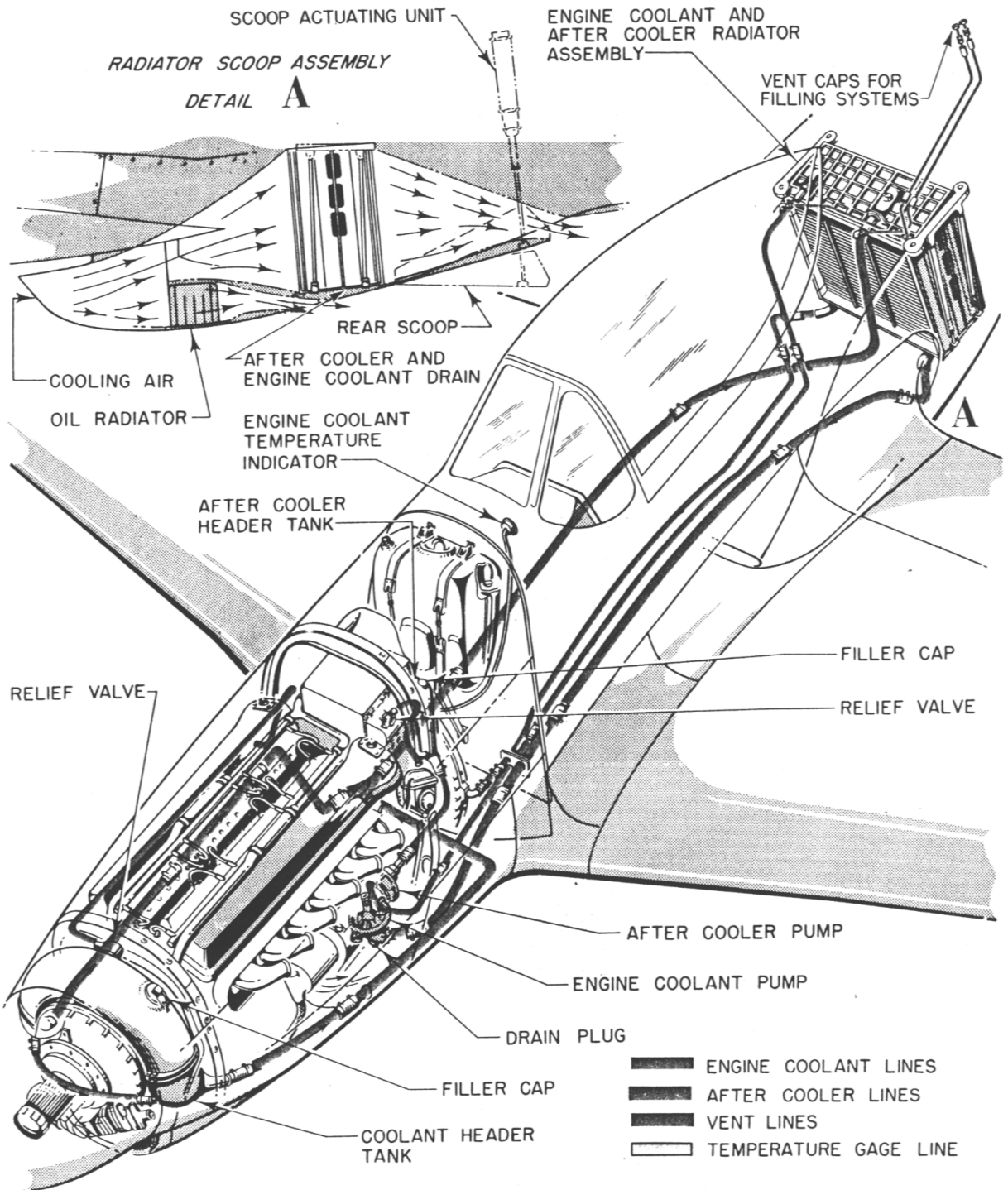
Figure 11—Cooling Systems
