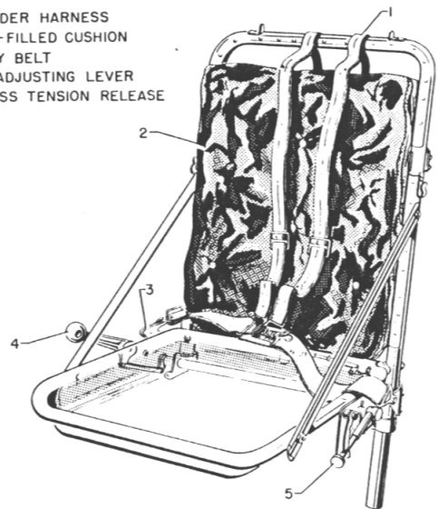
Figure 13—Pilot's Seat
