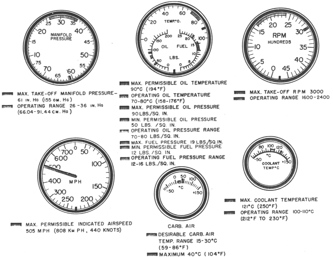
Figure 22—Instrument Limitations
