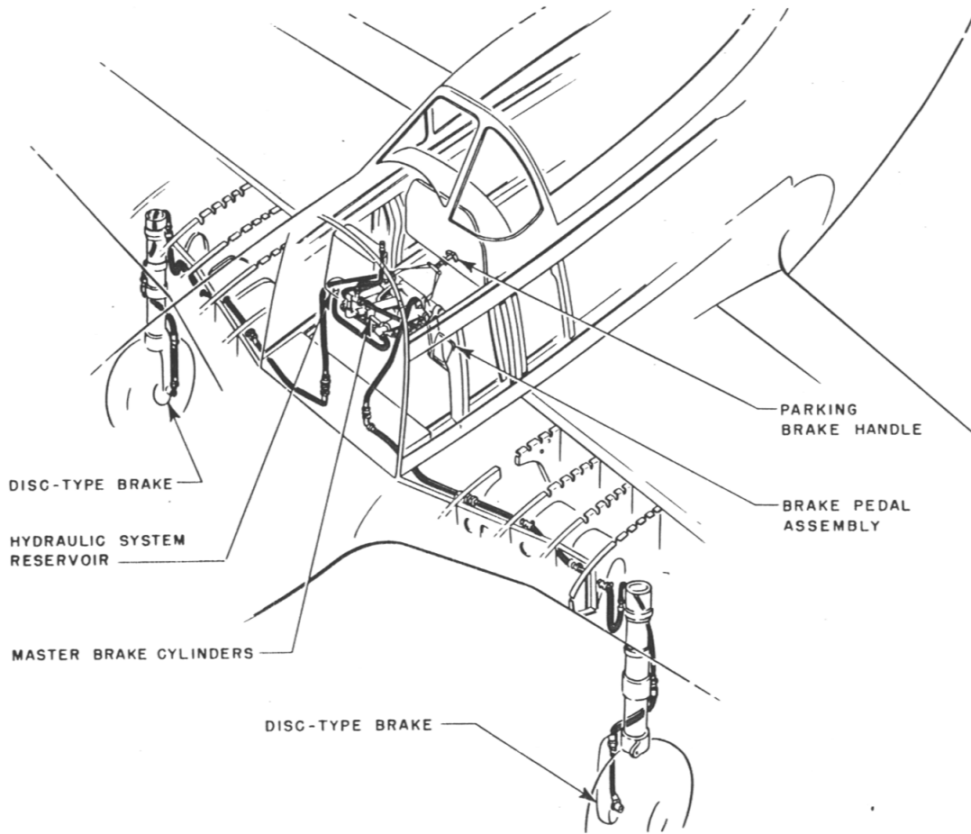
Figure 5—Brake System
