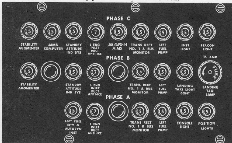
LEFT CONSOLE – REAR COCKPIT (Normally powered by left AC bus)
