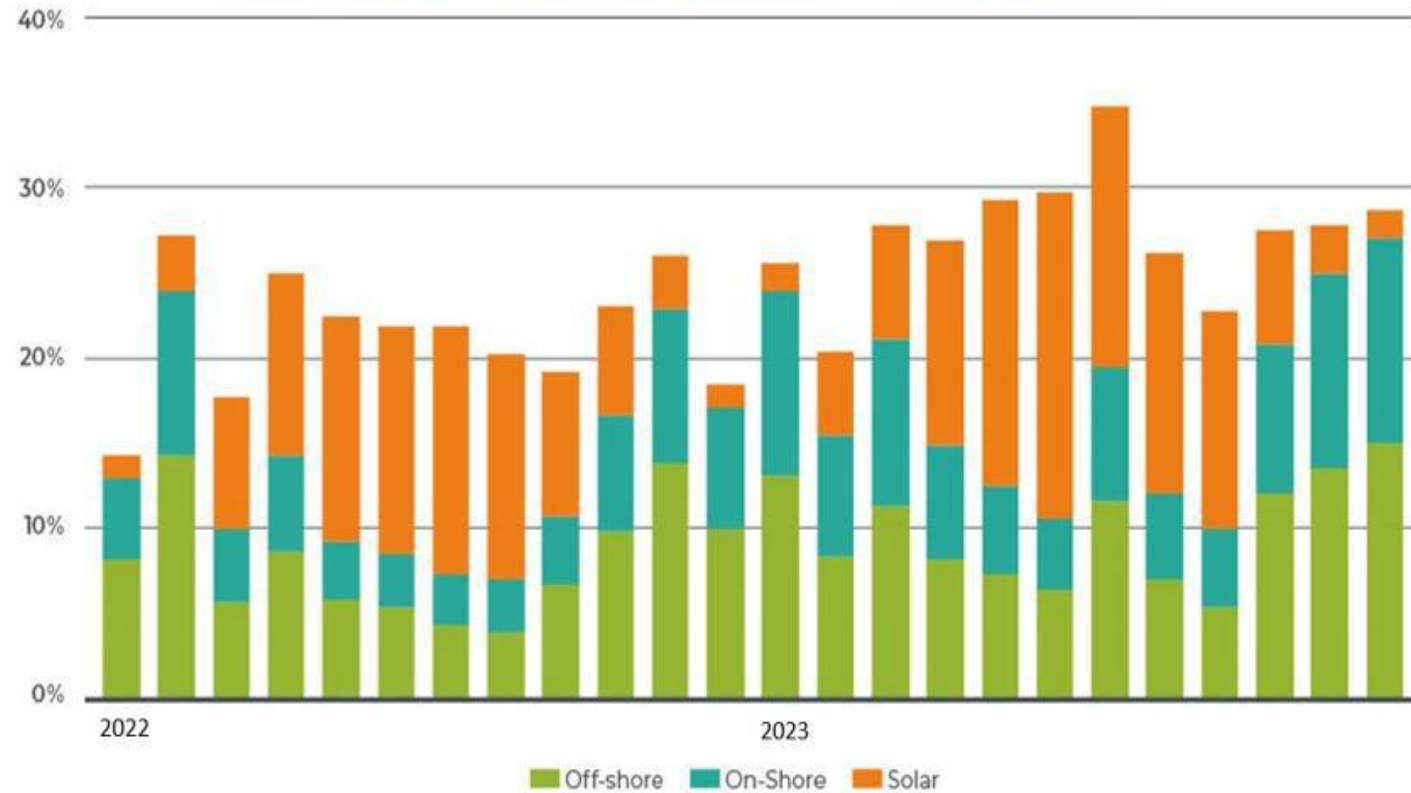
Monthly share of wind and solar production w.r.t. total load in Belgium
