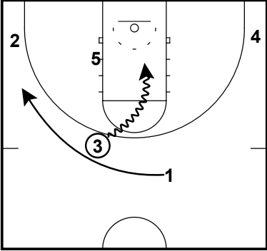
Fake handoff
