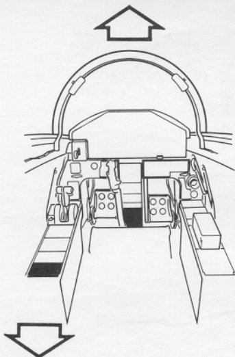
LEFT CONSOLE – FRONT COCKPIT
